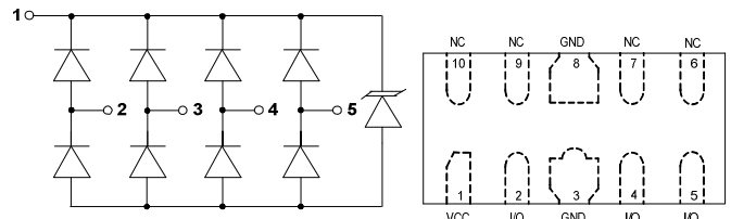
Circuit Diagram
